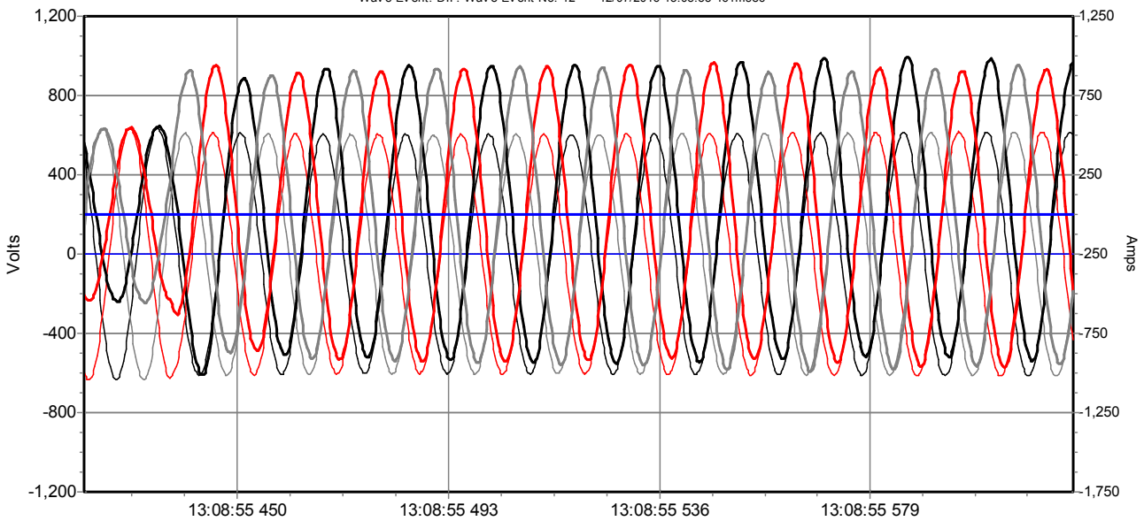
Wave Event: DIP. Wave Event No. 12 --- 12/07/2016 13:08:55 461msec
