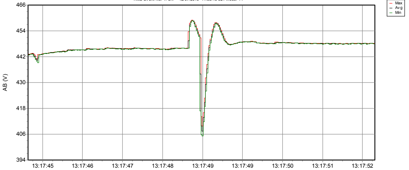
RMS Event No. 1: DIP 12/07/2016 11:53:18 521 msec. 14
