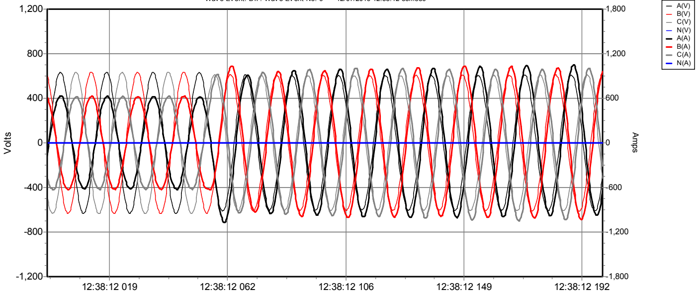
Wave Event: DIP. Wave Event No. 9 --- 12/07/2016 12:38:12 85msec
