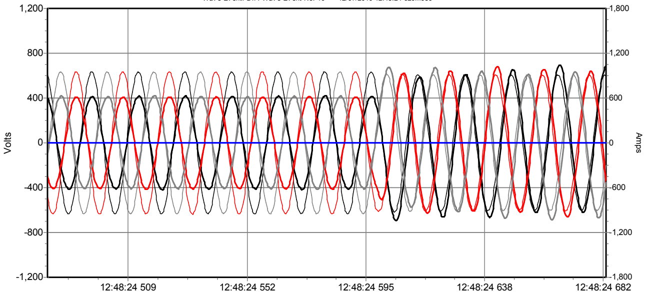
Wave Event: DIP. Wave Event No. 10 --- 12/07/2016 12:48:24 629msec
