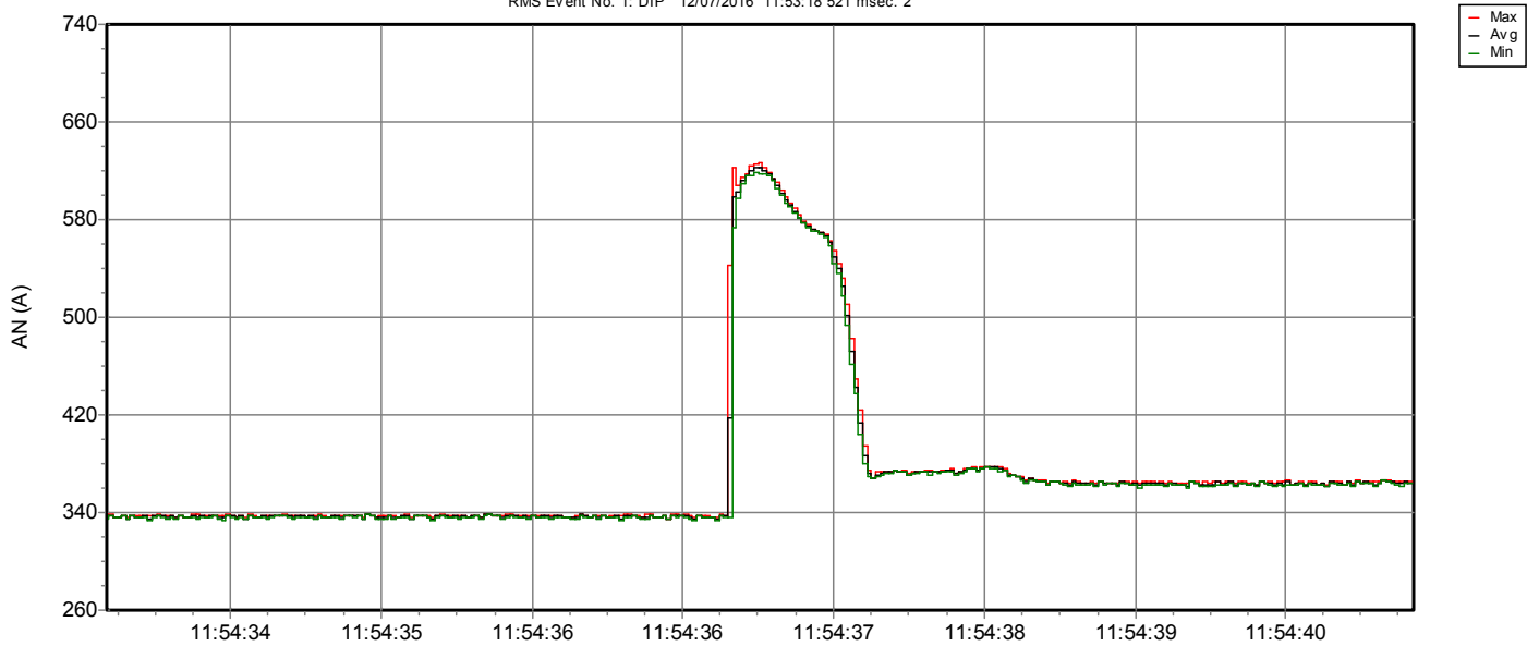
RMS Event No. 1: DIP 12/07/2016 11:53:18 521 msec. 2
