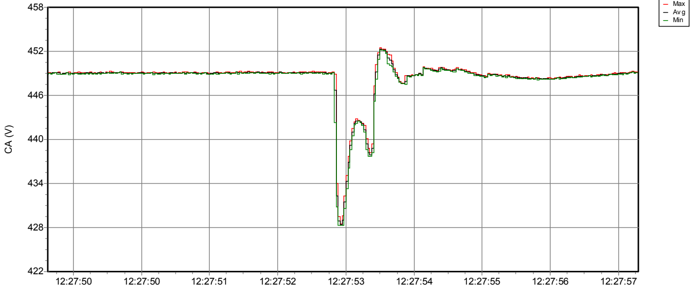
RMS Event No. 1: DIP 12/07/2016 11:53:18 521 msec. 8
