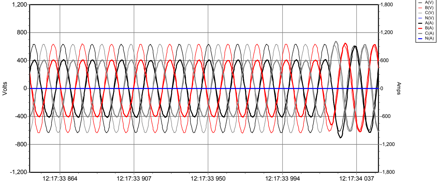
Wave Event: DIP. Wave Event No. 7 --- 12/07/2016 12:17:34 49msec
