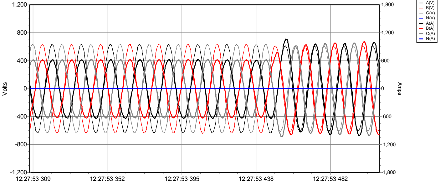
Wave Event: DIP. Wave Event No. 8 --- 12/07/2016 12:27:53 477msec
