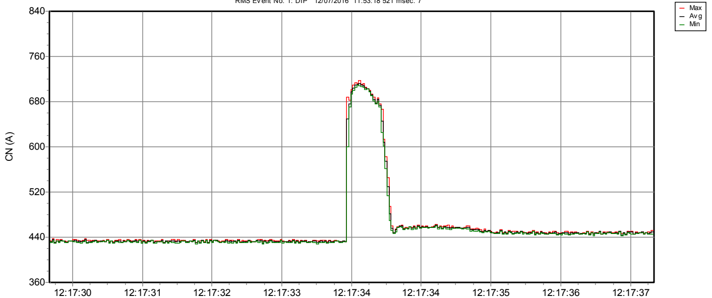
RMS Event No. 1: DIP 12/07/2016 11:53:18 521 msec. 7
