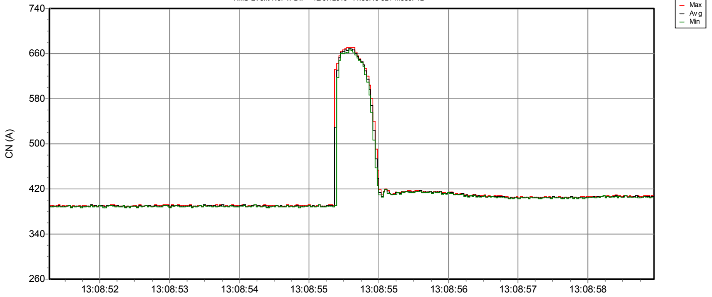
RMS Event No. 1: DIP 12/07/2016 11:53:18 521 msec. 12
