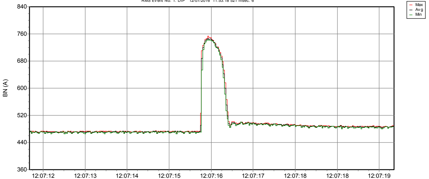
RMS Event No. 1: DIP 12/07/2016 11:53:18 521 msec. 6
