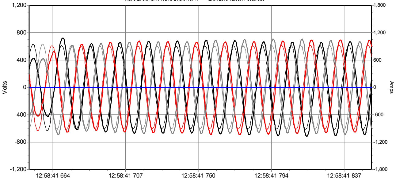
Wave Event: DIP. Wave Event No. 11 --- 12/07/2016 12:58:41 688msec
