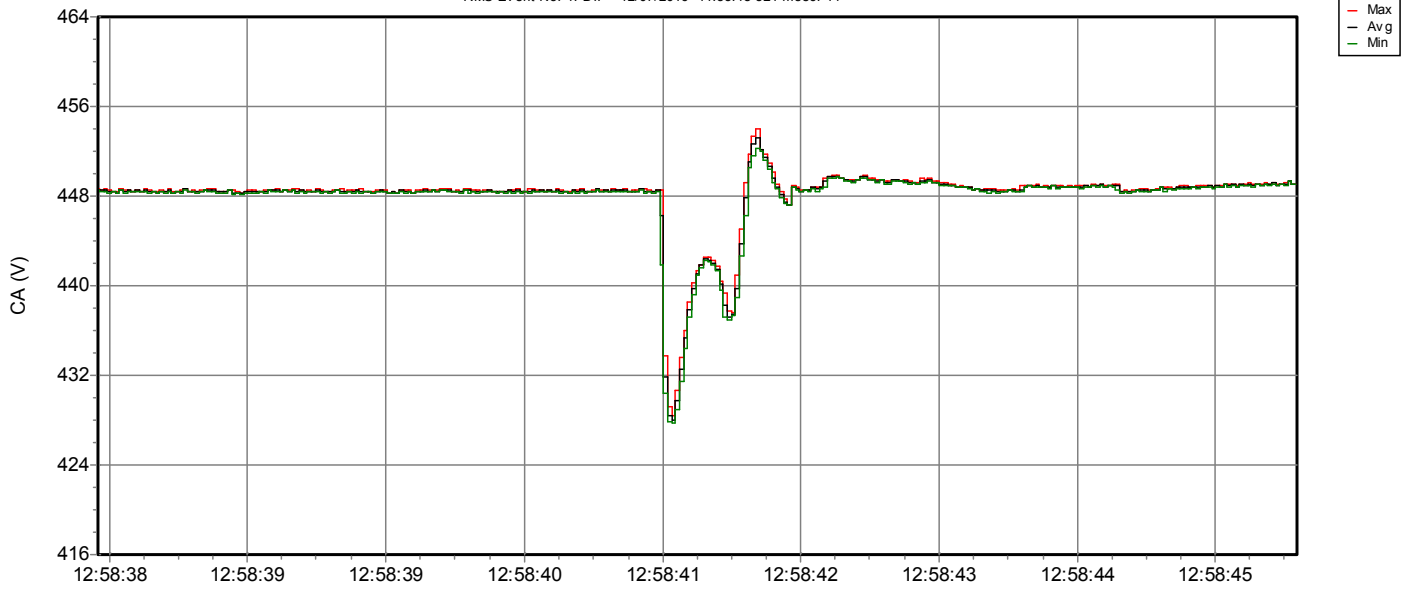
RMS Event No. 1: DIP 12/07/2016 11:53:18 521 msec. 11
