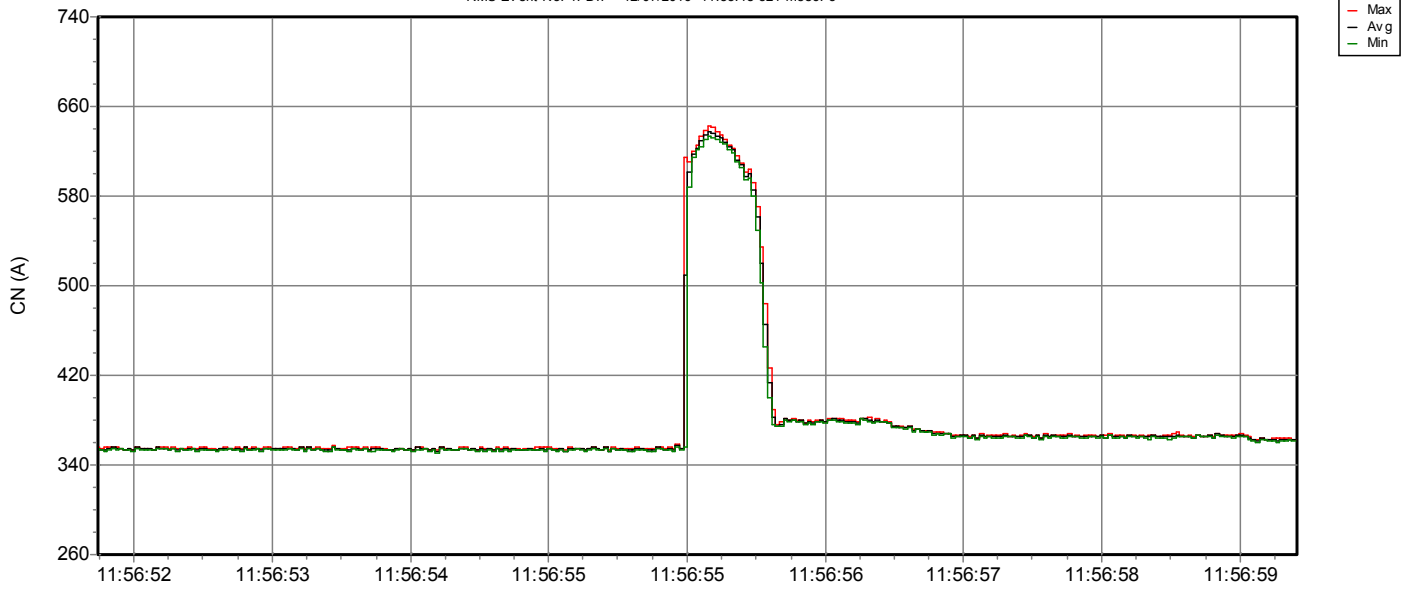
RMS Event No. 1: DIP 12/07/2016 11:53:18 521 msec. 3
